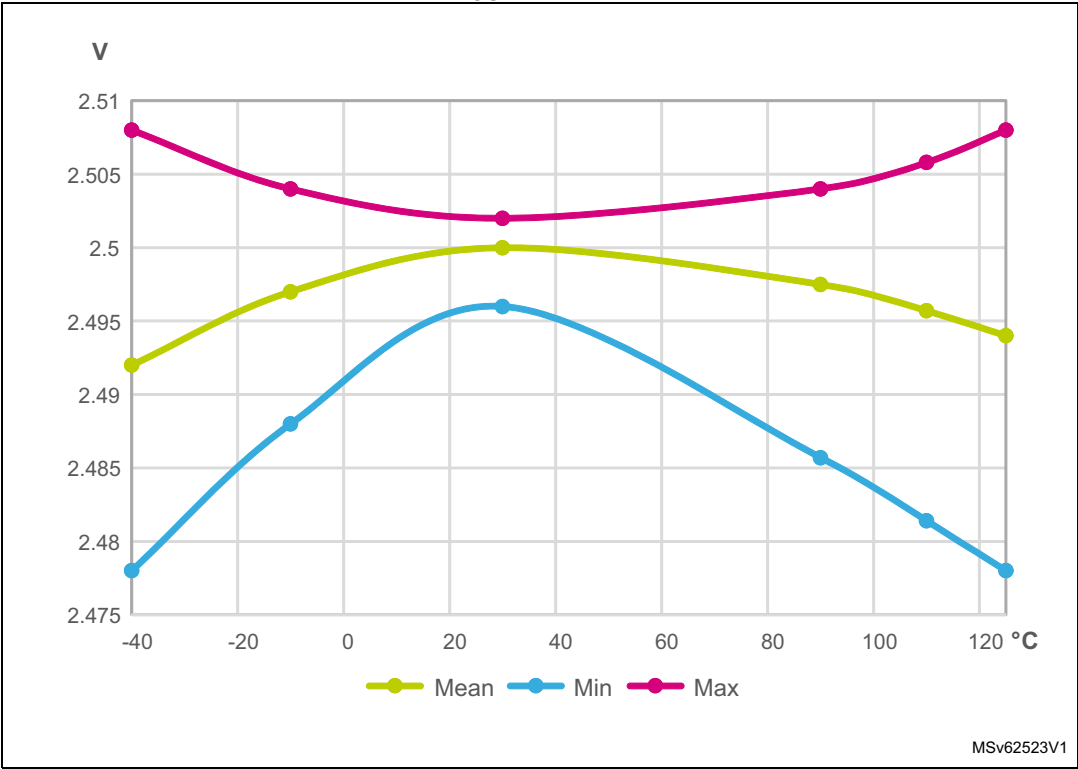
Figure 31. V_{\text{REFOUT}} \text{ TEMP} in case \text{VRS} = 01
