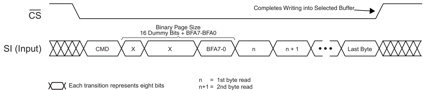
Figure 23-2. Buffer Write
