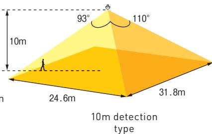
Standard detection type Slight motion detection type Spot detection type 10m detection type
