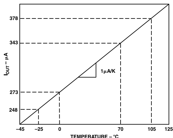
Figure 1. Transfer Characteristic
