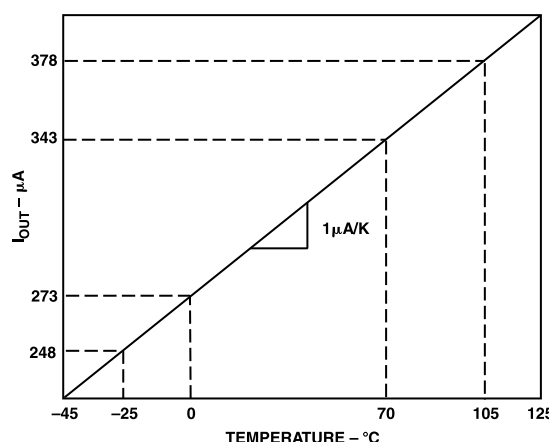
Figure 1. Transfer Characteristic
