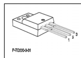
PG-TO220-3-31
