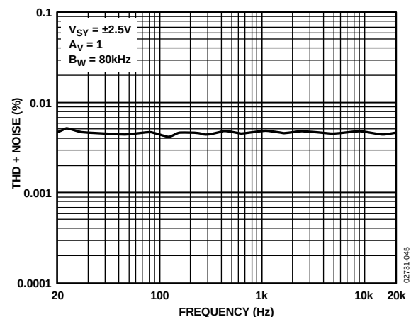
Figure 46. THD + Noise vs. Frequency
