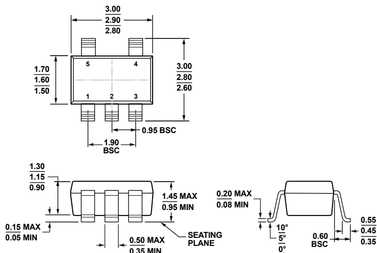
Figure 59. 5-Lead Small Outline Transistor Package [SOT-23] (RJ-5) Dimensions shown in millimeters
