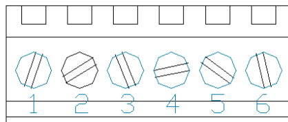
Figure 13: RS422 Header
