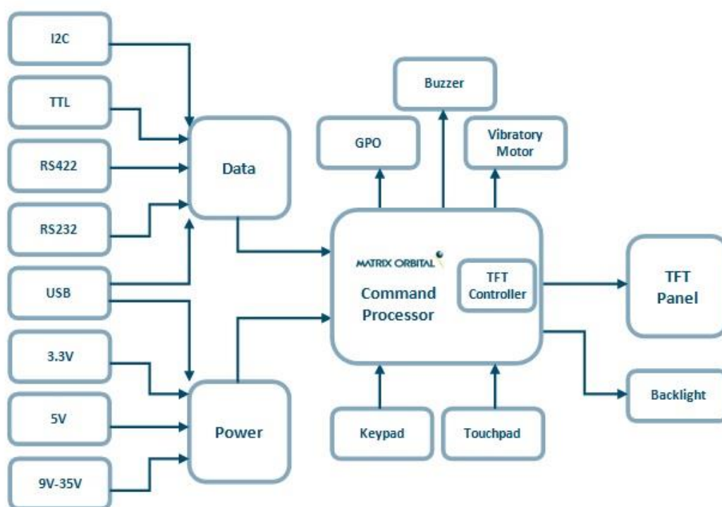
Figure 2: Functional Diagram
