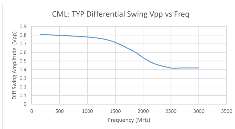
Figure 2.1. Typical Clock Output Swing Amplitudes vs. Frequency
