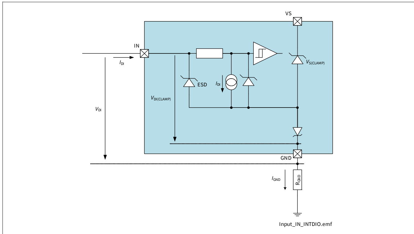
Figure 11 Input circuitry
