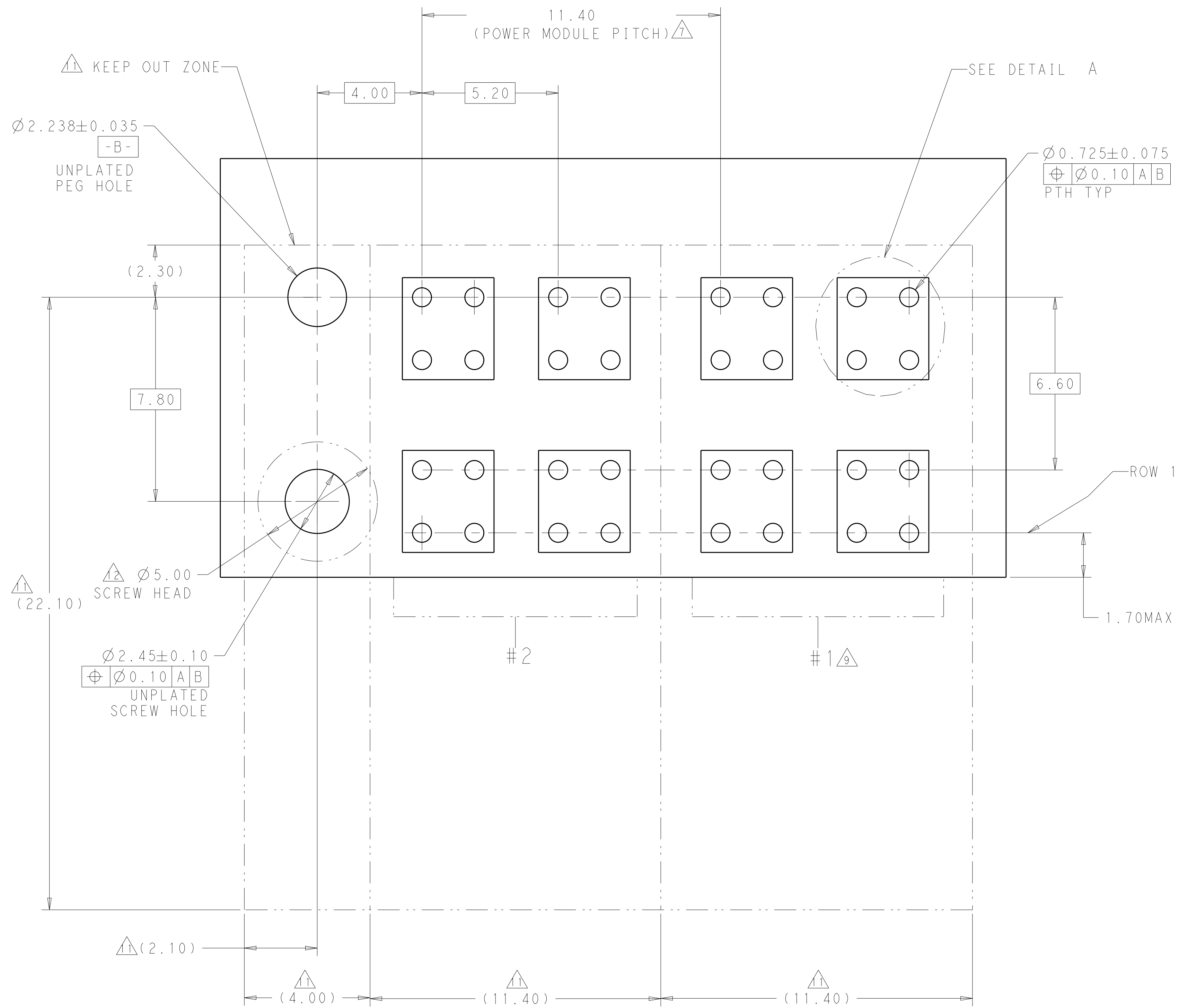
(2.00) 1.60 TO 4.40 PCB LAYOUT HOLD DOWN LEFT -2 POWER MODULE (COMPONENT SIDE SHOWN) (Ø 5.00) SCREW HEAD - A - THIS DRAWING IS A CONTROLLED DOCUMENT. OWN LERRY WANG 13FEB2012 STE IF C...
