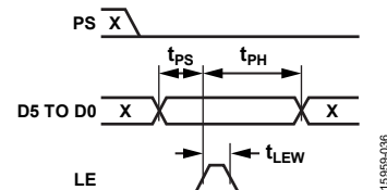
Figure 36. Latched Parallel Mode Timing Diagram
