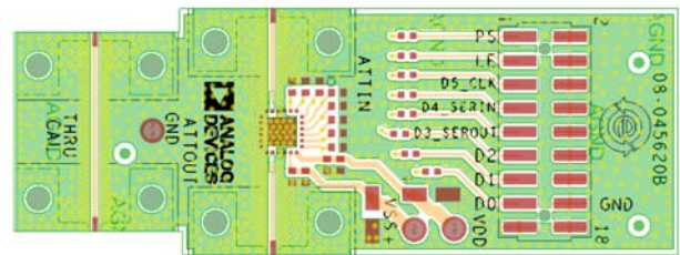
Figure 39. Evaluation Board, Top View
