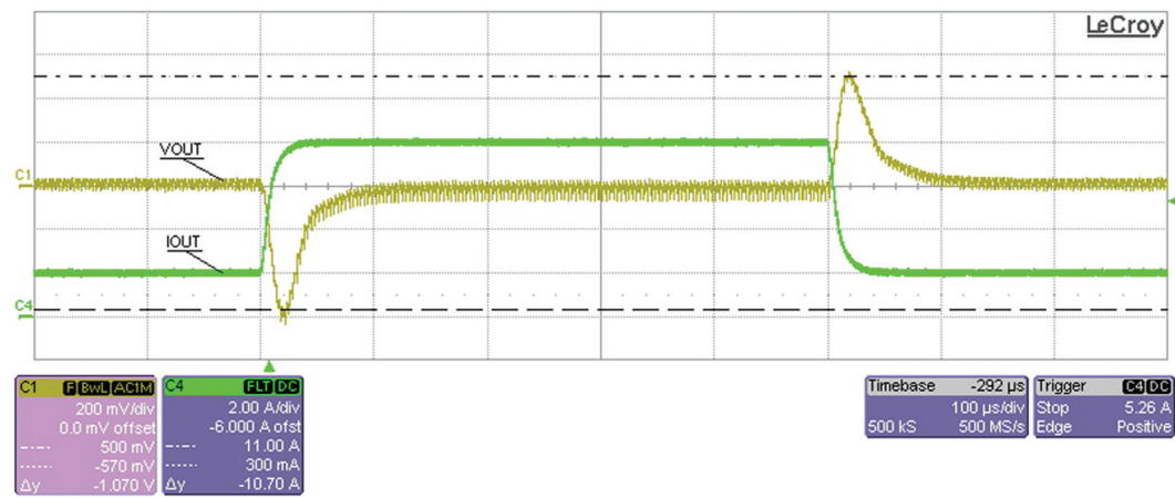
Figure 4. DC1619A 2A to 8A Load Transient
