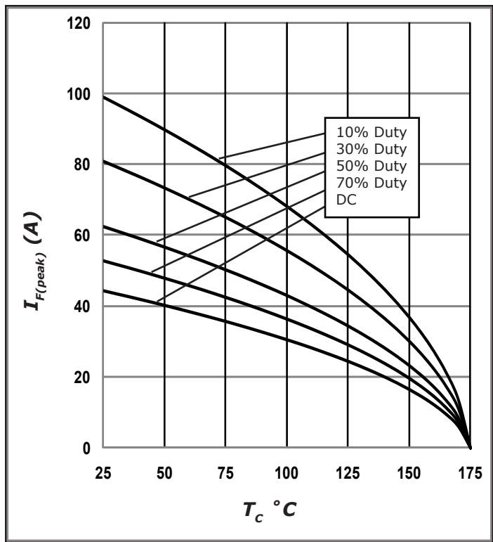
Figure 3. Current Derating
