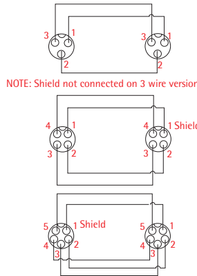
STANDARD WIRING FOR CONNECTOR CONFIGURATION 2 STANDARD WIRING FOR CONNECTOR CONFIGURATION 3, 4 AND 6
