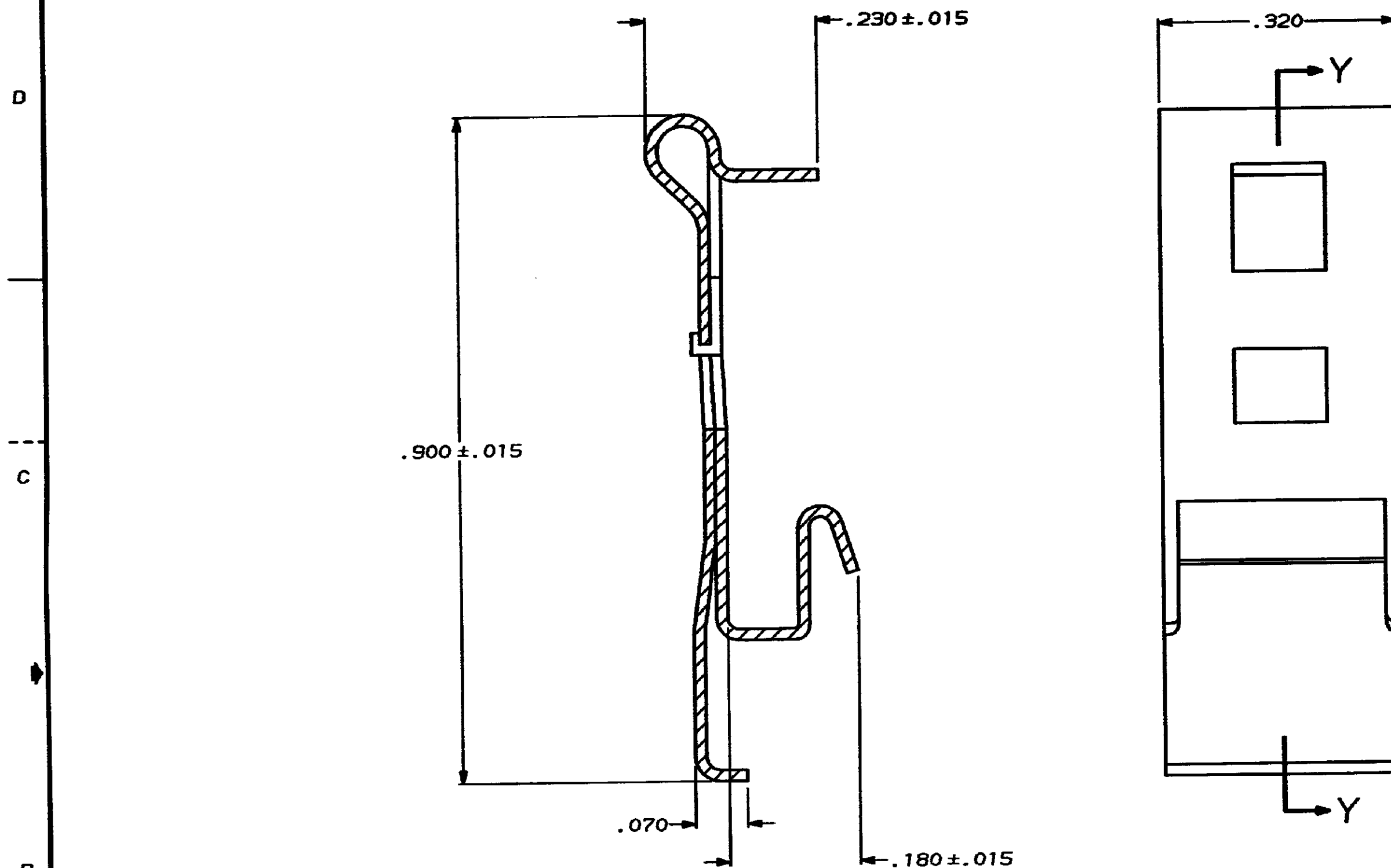
SECTION Y-Y
