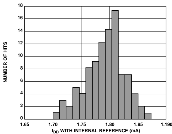
Figure 30. I_{DD} Histogram with Internal Reference
