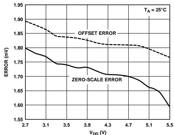
Figure 28. Zero-Scale Error and Offset Error vs. Supply Voltage
