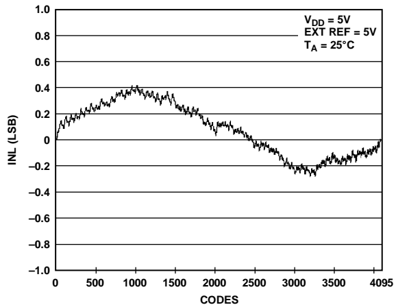
Figure 9. INL AD5628—External Reference
