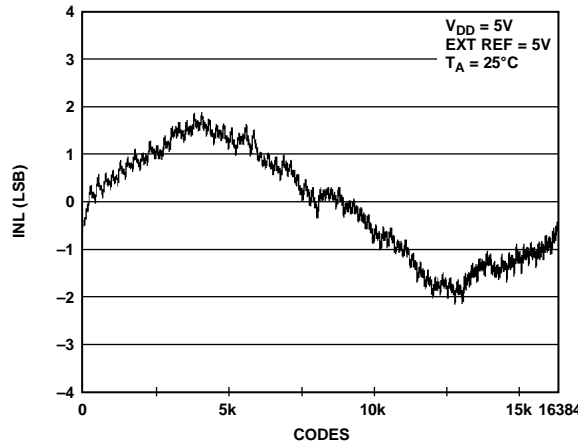
Figure 8. INL AD5648—External Reference
