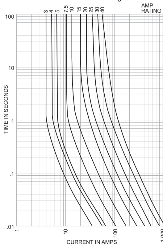
Time-Current Characteristic Curves - Average Melt
