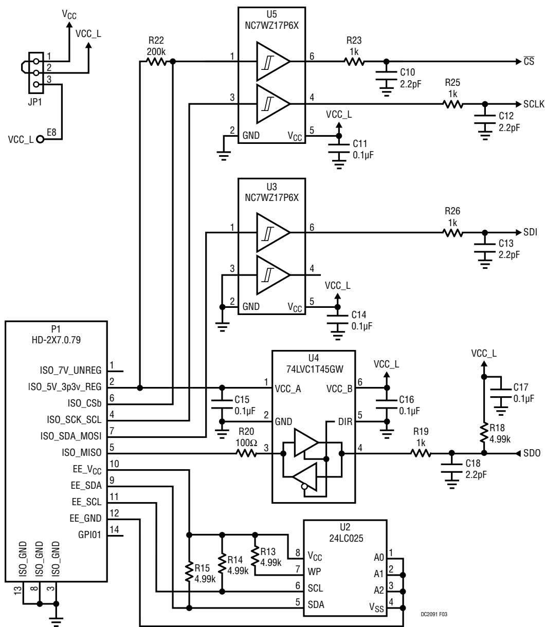
Figure 3. Demo Board SPI Interface
