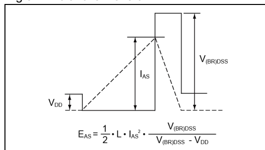
Fig.3-2 Avalanche Waveform
