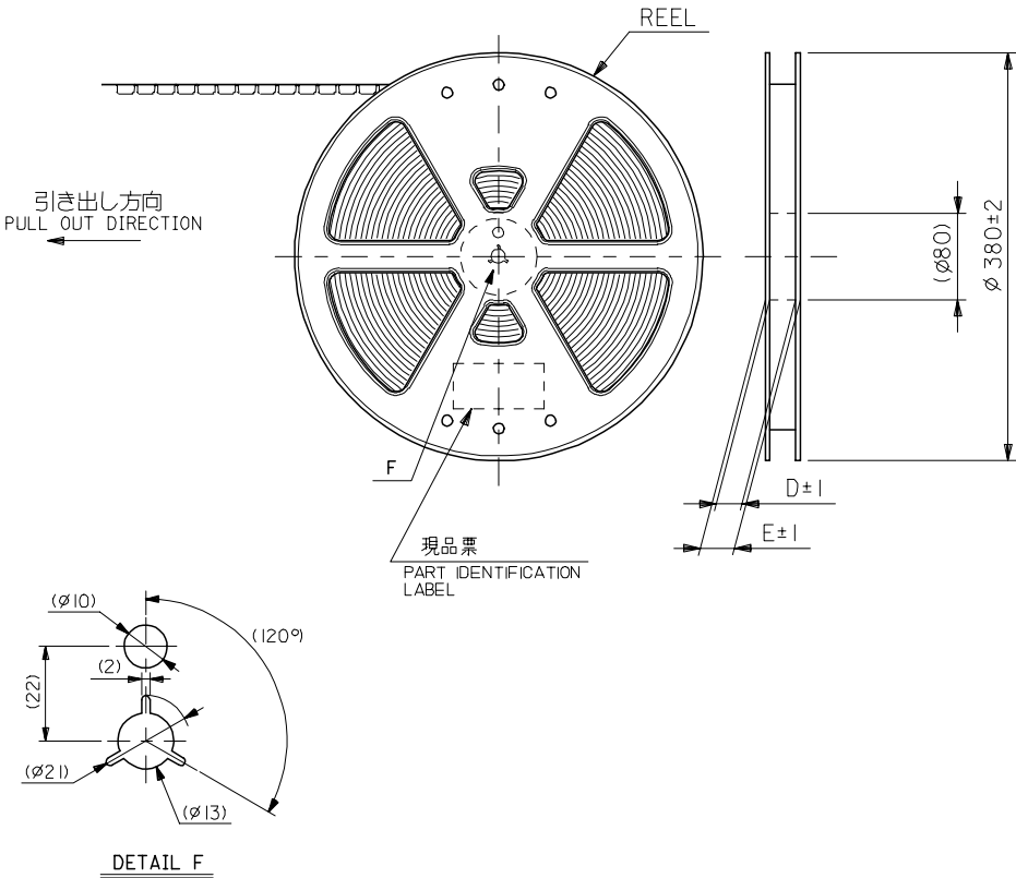
DETAIL F
