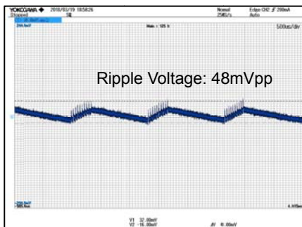
Figure 15. VOUT Ripple Voltage.1 V_{IN}=100Vac , I_{OUT}=10mA CH1: VOUT 50mV/div, 500µs/div
