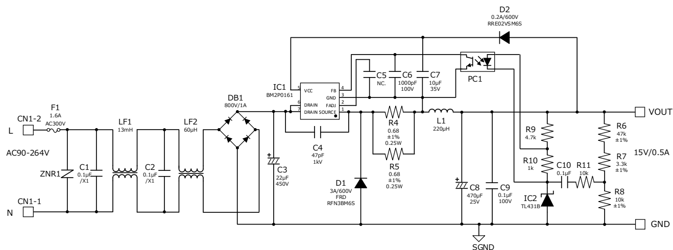
Figure 3. BM2P0161-EVK-001 Schematics
