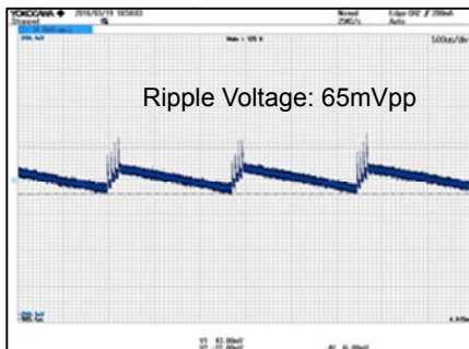
Figure 18. VOUT Ripple Voltage.4 V_{IN}=230Vac , I_{OUT}=10mA CH1: VOUT 50mV/div, 500µs/div
