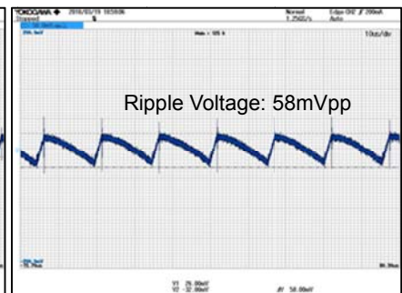
Figure 17. VOUT Ripple Voltage.3 V_{IN}=100Vac , I_{OUT}=500mA CH1: VOUT 50mV/div, 10µs/div
