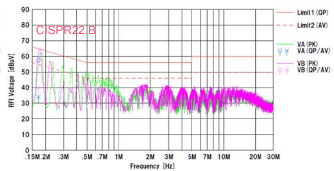
Figure 22. Conducted Emission.2
