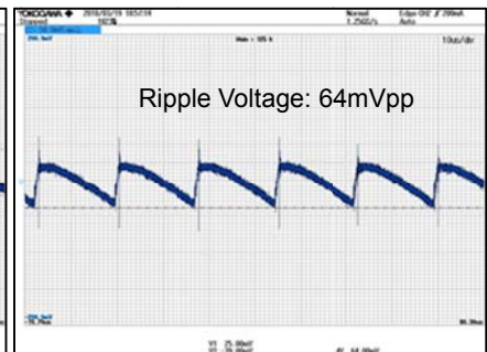
Figure 20. VOUT Ripple Voltage.6 V_{IN}=230Vac , I_{OUT}=500mA CH1: VOUT 50mV/div, 10µs/div
