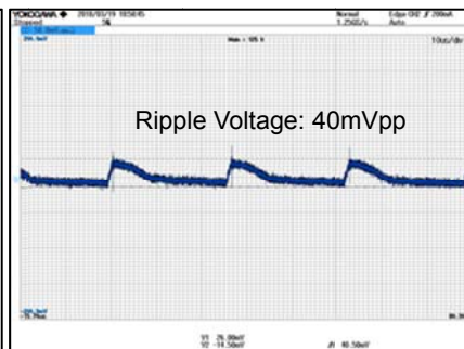
Figure 16. VOUT Ripple Voltage.2 V_{IN}=100Vac , I_{OUT}=100mA CH1: VOUT 50mV/div, 10µs/div
