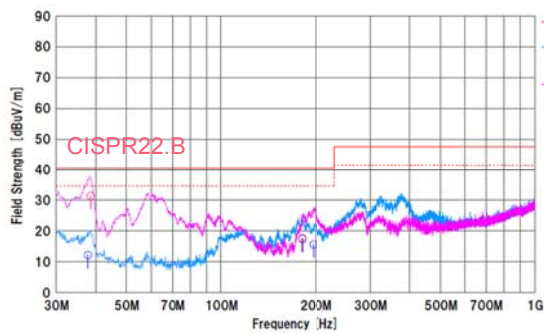
Figure 23. Radiated Emission.1
