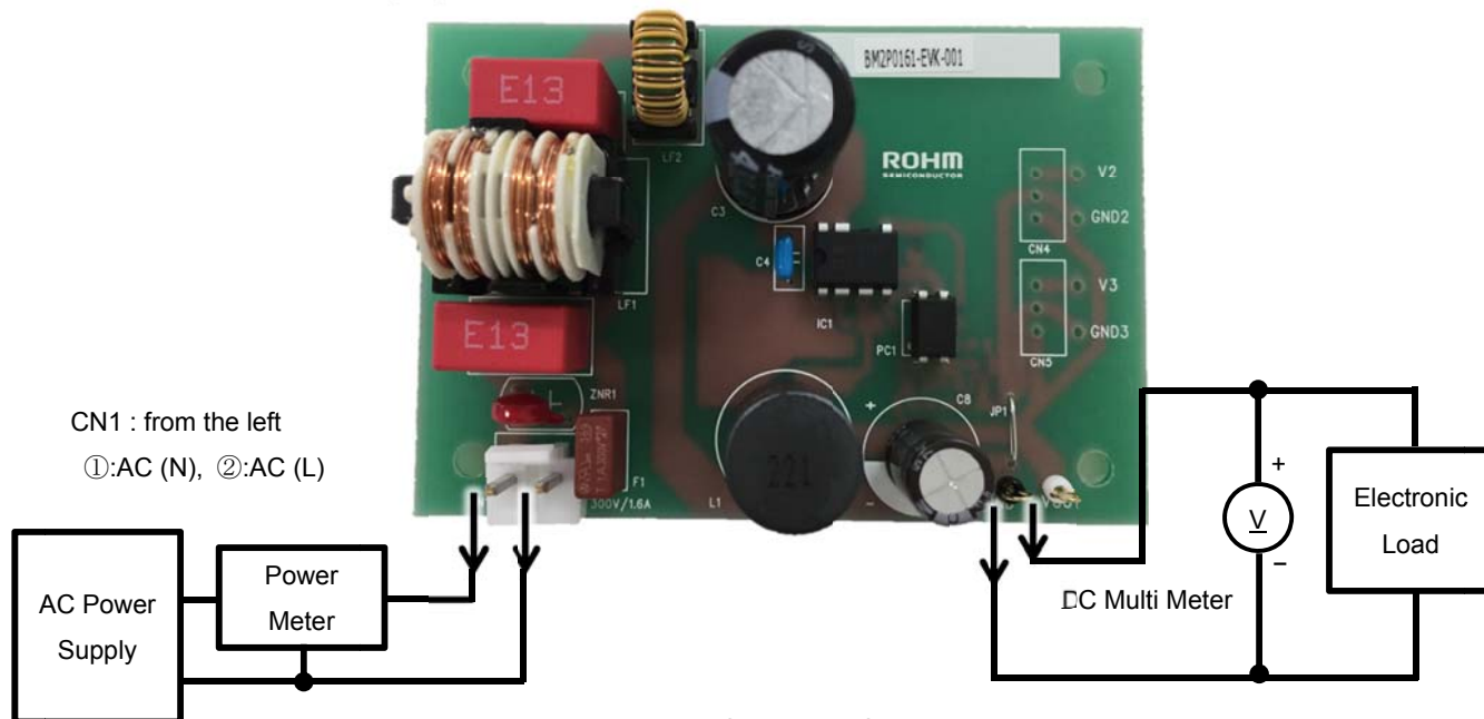
Figure 1. Connection Circuit
