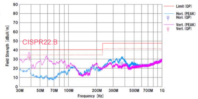
Figure 24. Radiated Emission.2
