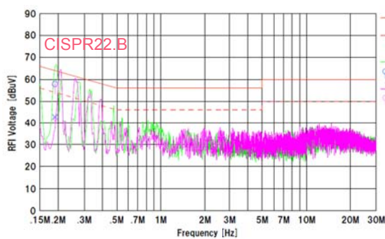
Figure 21. Conducted Emission.1
