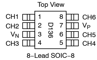
PACKAGE / PINOUT DIAGRAMS
