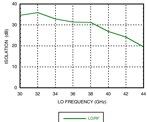
LO/RF isolation
