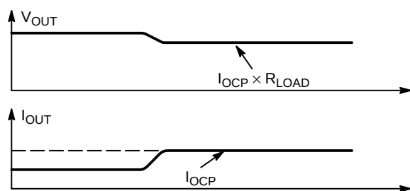
Figure 23. Overload
