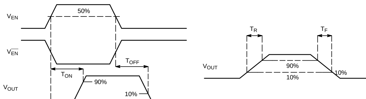
Figure 4. Voltage Waveform
