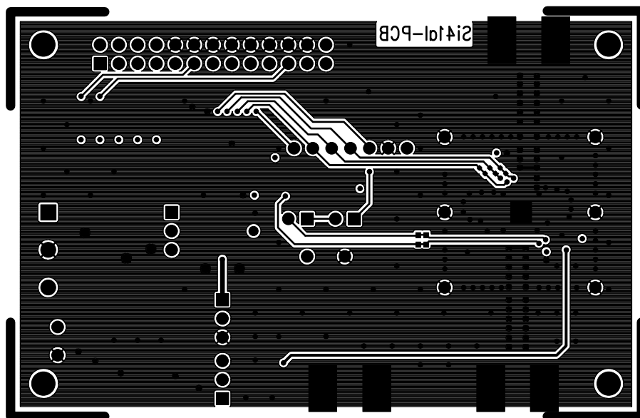
Figure 30. Si4133M Solder
