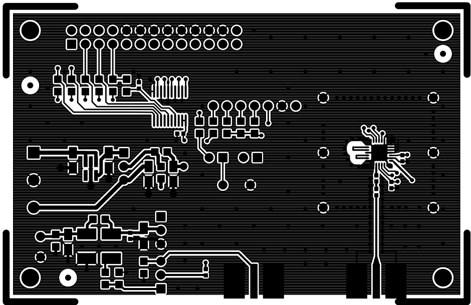
Figure 32. Si4113GX5-BM Component
