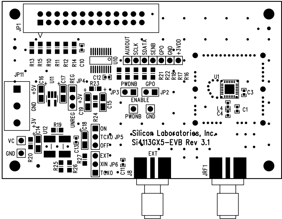
Figure 31. Si4113GX5-BM Silkscreen
