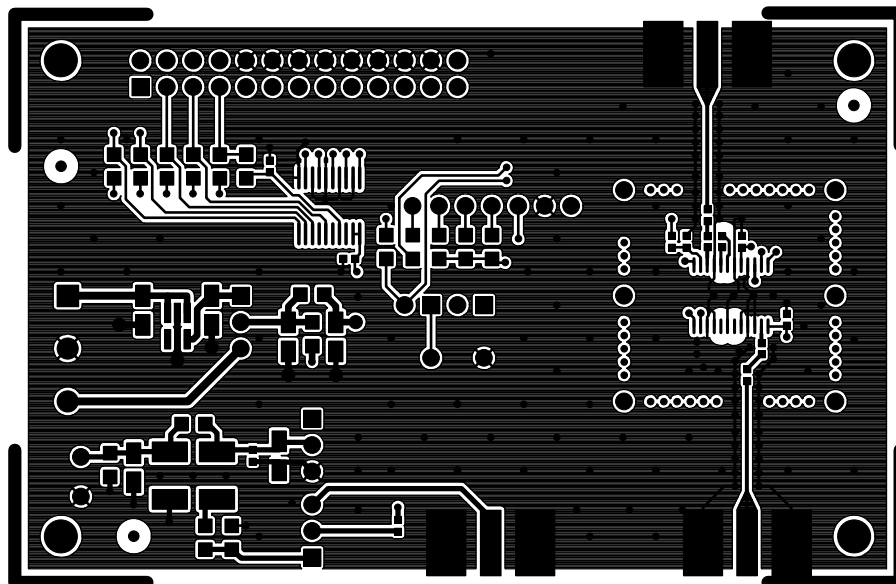
Figure 42. Si4136BT Component
