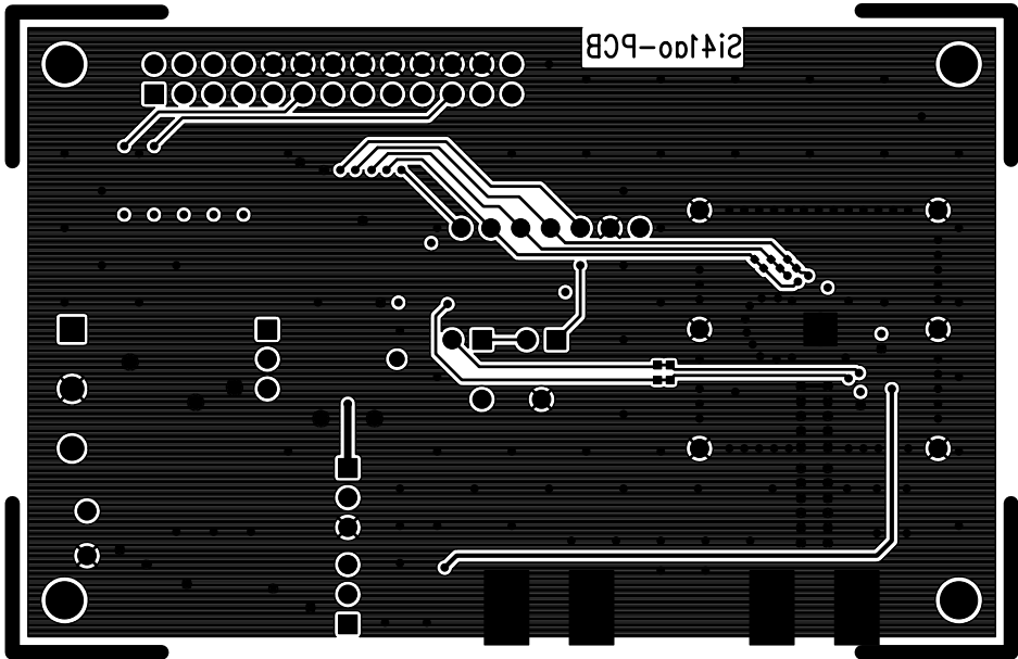
Figure 35. Si4113GX5-BM Solder
