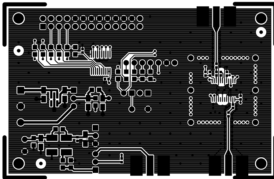
Figure 42. Si4136BT Component
