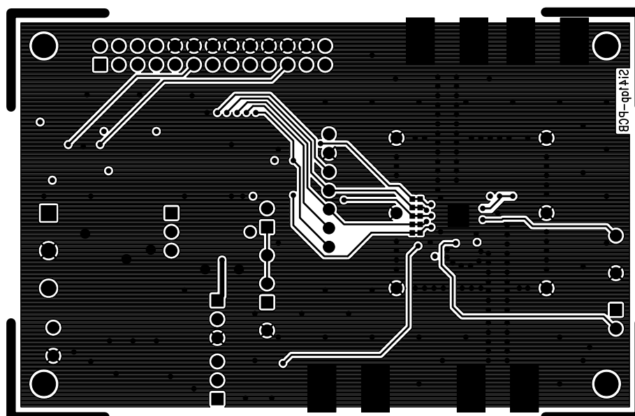
Figure 40. Si4135M Solder
