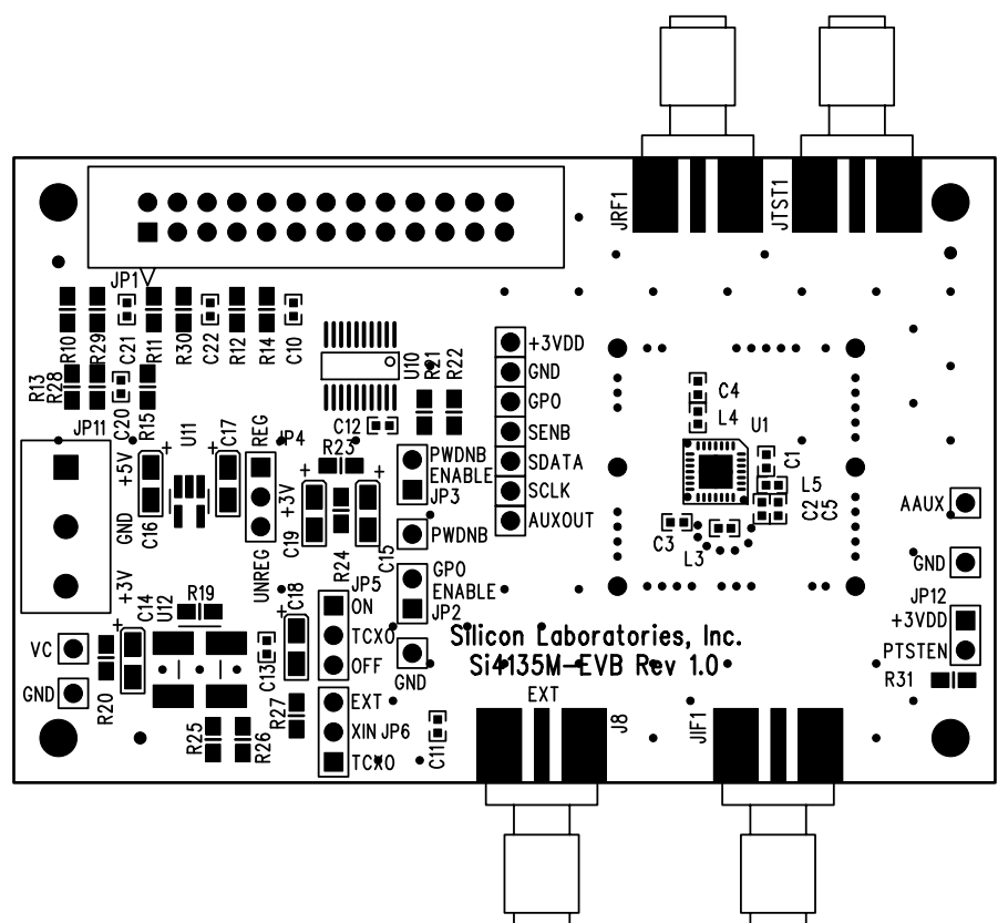
Figure 36. Si4135M Silkscreen
