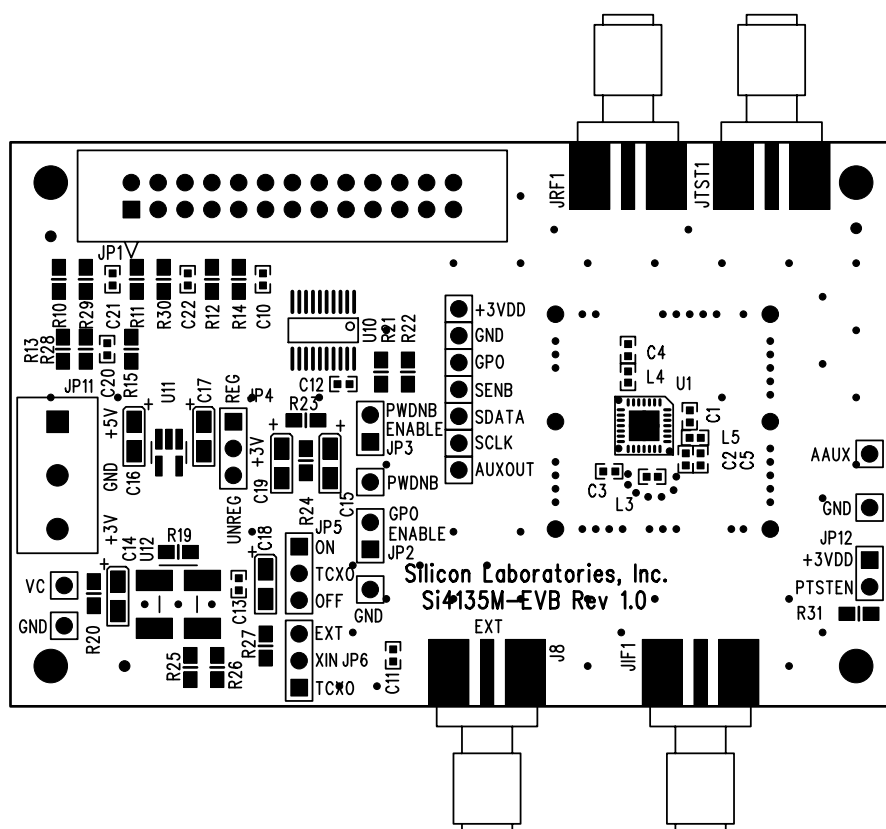
Figure 36. Si4135M Silkscreen
