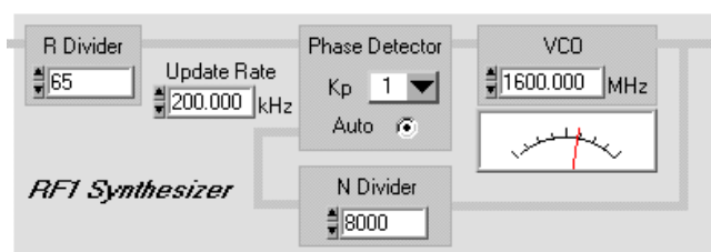
Figure 7. VCO Tuning
