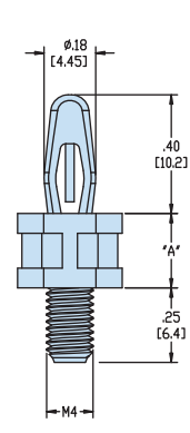
BAYONET SNAP LOCK 10,2 / M4 MALE THREAD
