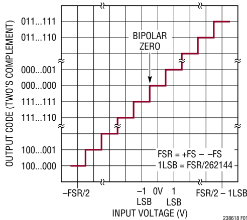
Figure 1. LTC2386-18 Transfer Function
