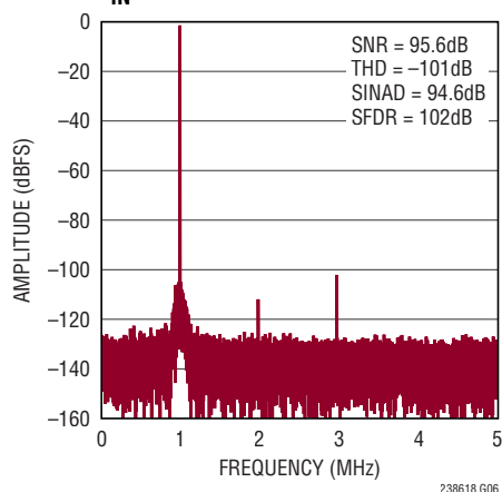
32k Point FFT f_{\text{SAMPL}} = 10\text{Mps} , f_{\text{IN}} = 1\text{MHz}
