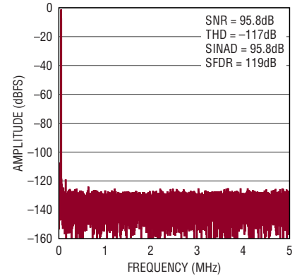
32k Point FFT, f_{\text{SAMPL}} = 10\text{Msps} , f_{\text{IN}} = 50\text{kHz}
