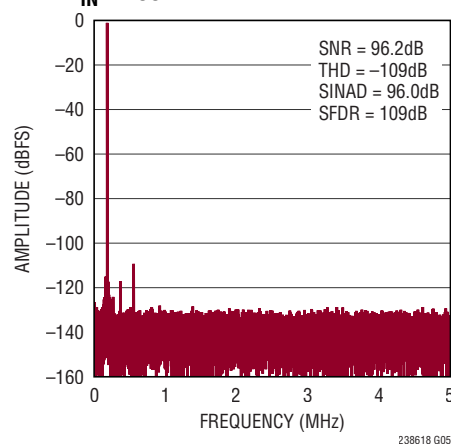
32k Point FFT f_{\text{SAMPL}} = 10\text{Mps} , f_{\text{IN}} = 200\text{kHz}
