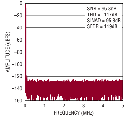
32k Point FFT, f_{\text{SAMPL}} = 10\text{Mps} , f_{\text{IN}} = 50\text{kHz}
