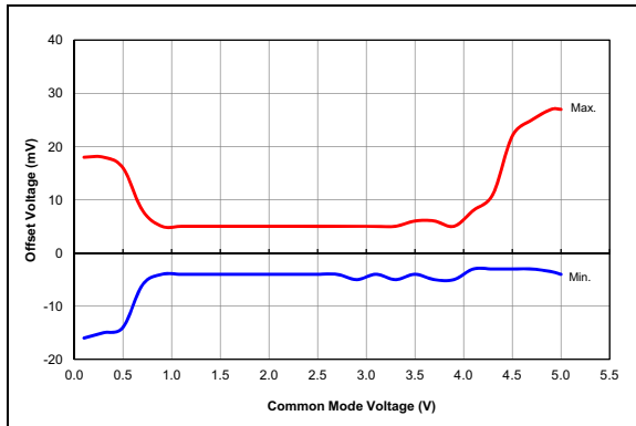
FIGURE 36-91: Comparator Offset, NP Mode ( C_{xSP} = 1 ), V_{DD} = 5.5V , Typical Measured Values From -40^\circ C to 125^\circ C , PIC16F1615/9 Only.
