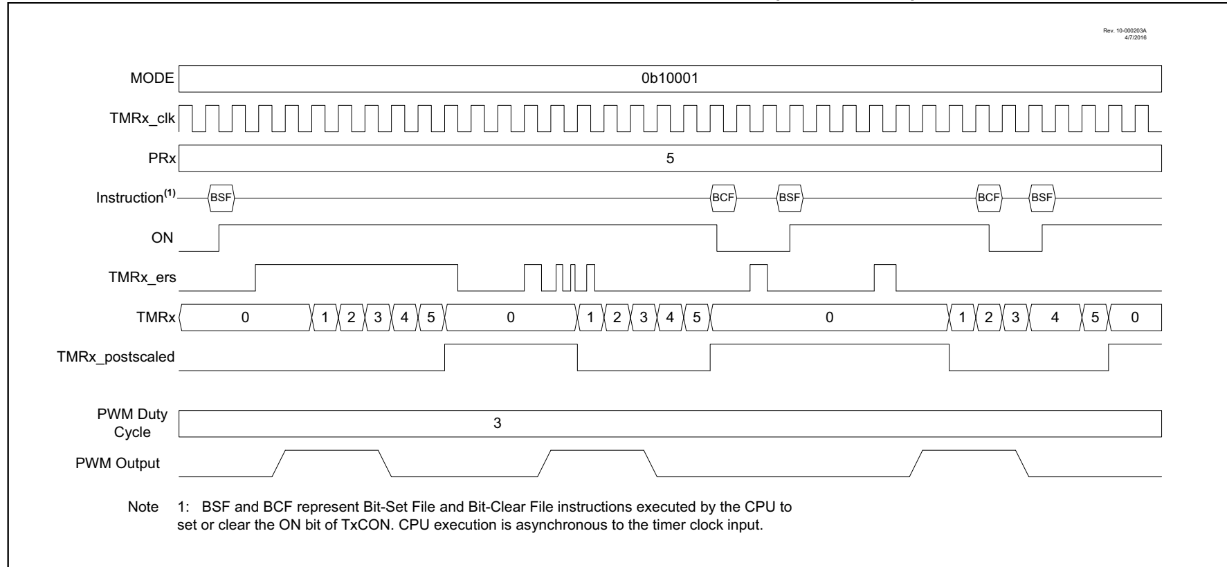
FIGURE 23-12: RISING EDGE-TRIGGERED MONOSTABLE MODE TIMING DIAGRAM (MODE = 10001)
