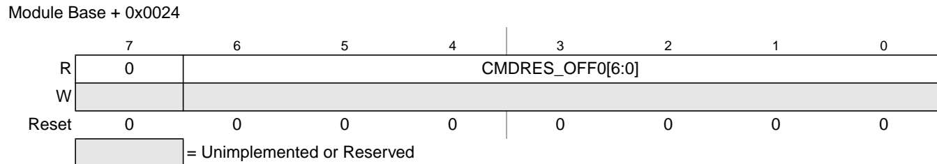
Figure 9-26. ADC Command and Result Offset Register 0 (ADCCROFF0)
