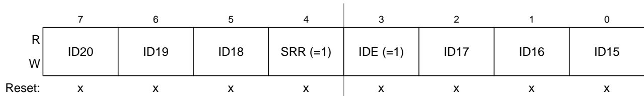
Figure 12-27. Identifier Register 1 (IDR1) — Extended Identifier Mapping
