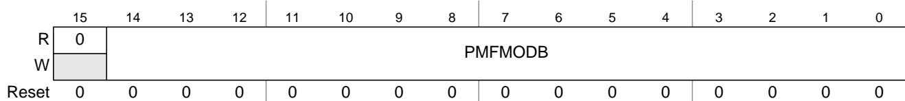
Figure 14-32. PMF Counter Modulo B Register (PMFMOBDB)
