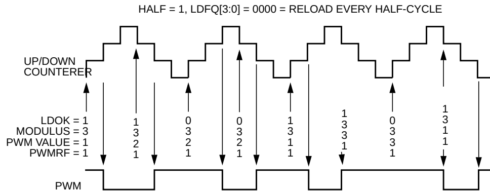
Figure 14-78. Half-Cycle Center-Aligned PWM Value Loading
