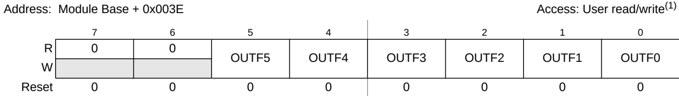
Figure 14-40. PMF Output Control on Fault Register (PMFOUTF)
