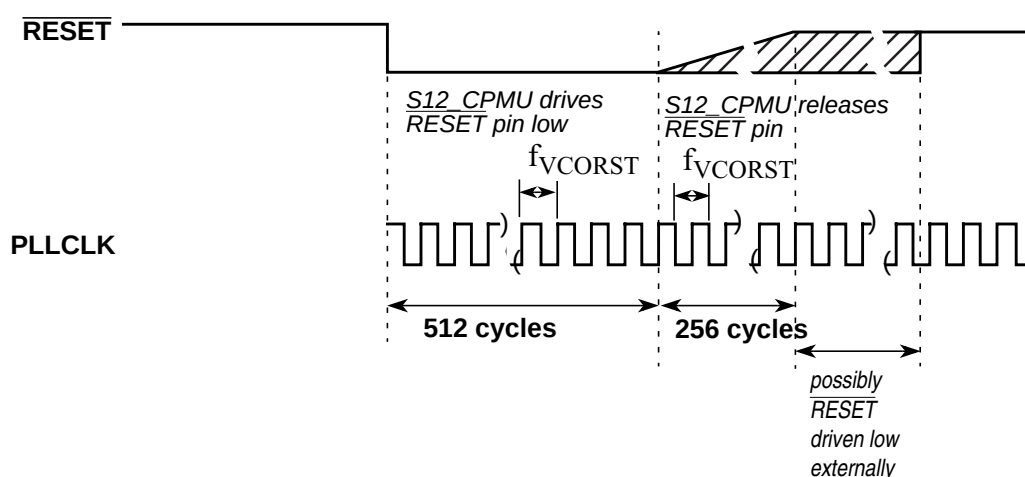
Figure 8-40. RESET Timing
