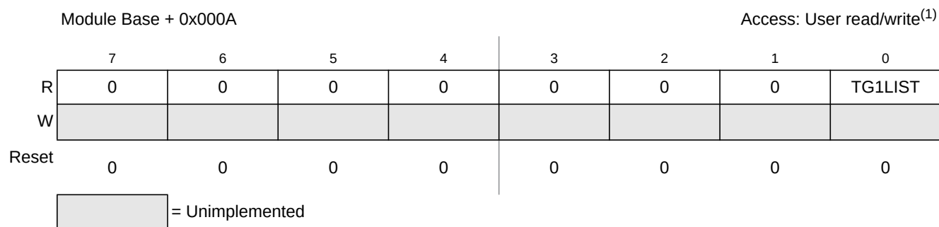
Figure 13-12. Trigger Generator 1 List Register (TG1LIST)
