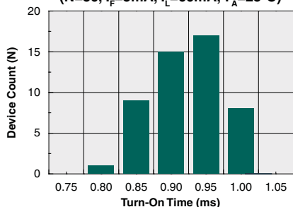
Typical Turn-On Time ( N=50 , I_F=5\text{mA} , I_L=60\text{mA} , T_A=25^\circ\text{C} )
