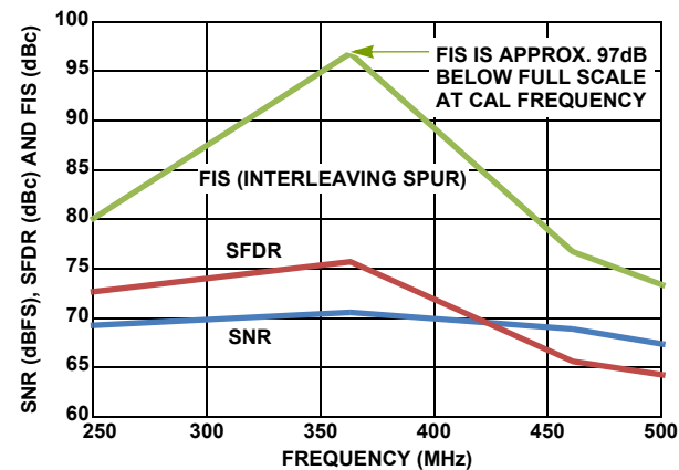
FIGURE 19. INPUT FREQUENCY SWEEP WITH I2E FROZEN, I2E PREVIOUSLY CALIBRATED AT 363MHz
