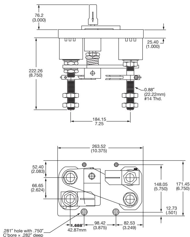
Dimensional Data 15200-609
