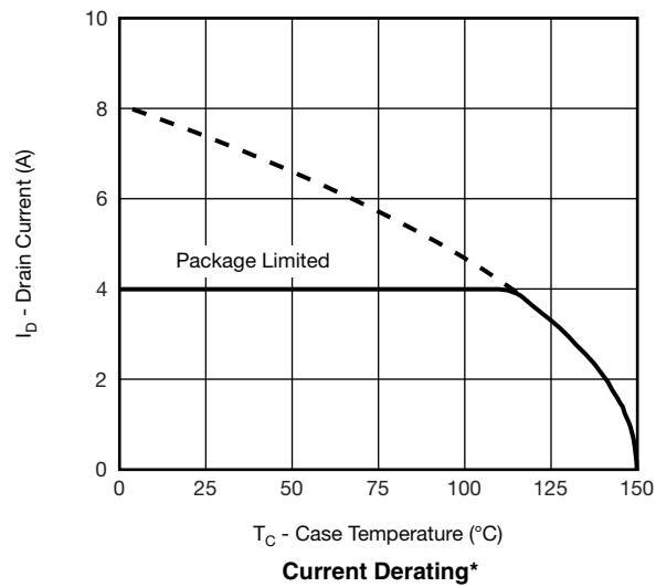
Current Derating*
