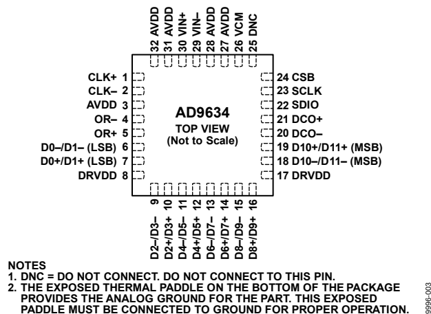
Figure 3. Pin Configuration
