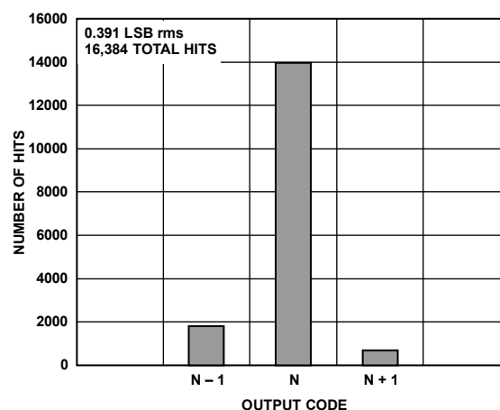
Figure 27. AD9634-210 Grounded Input Histogram, f_s = 210 MSPS
