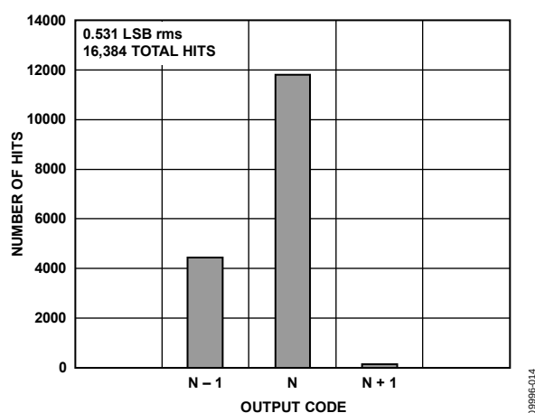
Figure 15. AD9634-170 Grounded Input Histogram, f_s = 170 MSPS
