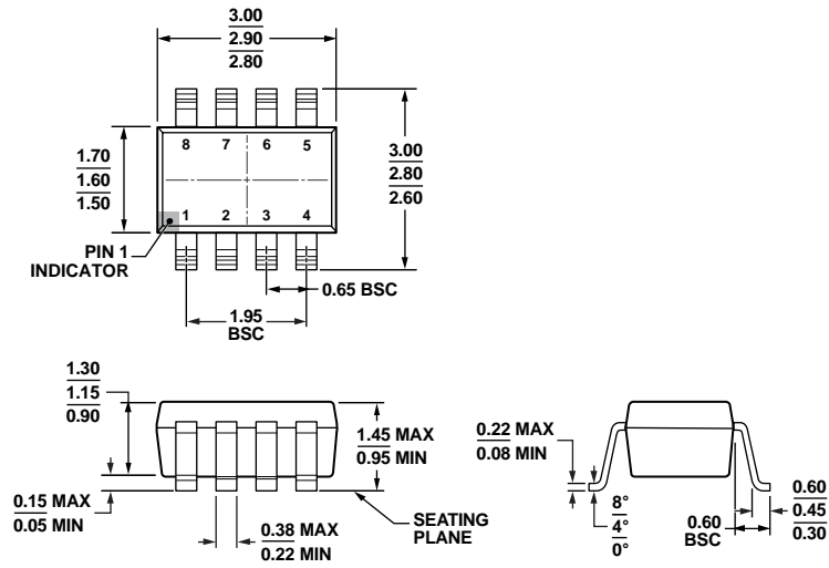
Figure 30. 8-Lead Small Outline Transistor Package [SOT-23] (RJ-8)
